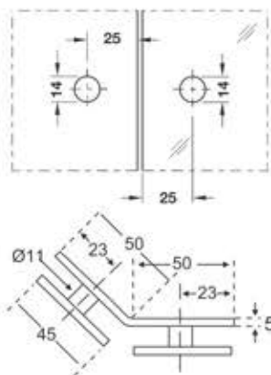
ZGC-33 Glass to Glass 90° M.R.P ₹ 592.00 (Matt) M.R.P ₹ 676.00 (Glossy)
