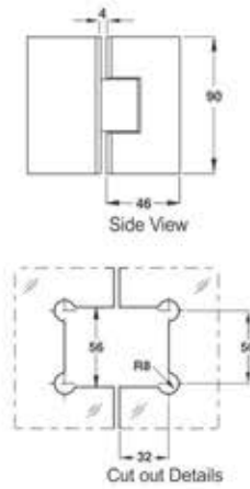
ZSH-03 Glass to Glass Hinge 135° M.R.P ₹ 3234.00 (Matt) M.R.P ₹ 3234.00 (Glossy)
