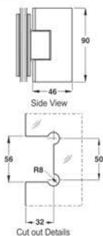
ZSH-55 Wall to Glass Hinge 90° Fix Bracket M.R.P ₹ 1014.00 (Matt) M.R.P ₹ 1014.00 (Glossy)
