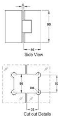
ZSH-33 Glass to Glass Hinge 135° M.R.P ₹ 1637.00 (Matt) M.R.P ₹ 1637.00 (Glossy)
