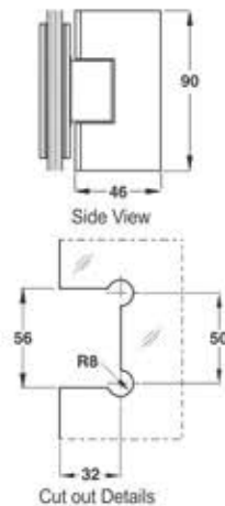
ZSH-05 Wall to Glass Hinge 90° Fix Bracket M.R.P ₹ 1691.00 (Matt) M.R.P ₹ 1391.00 (Glossy)
