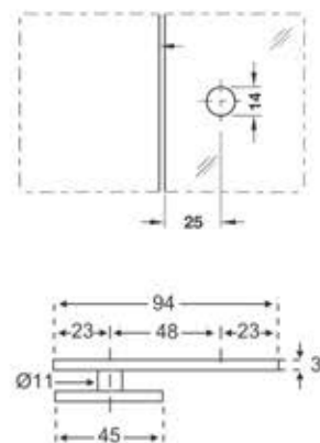
ZGC-07 T-Connector Glass to Glass 90° M.R.P ₹ 508.00 (Matt) M.R.P ₹ 578.00 (Glossy)
