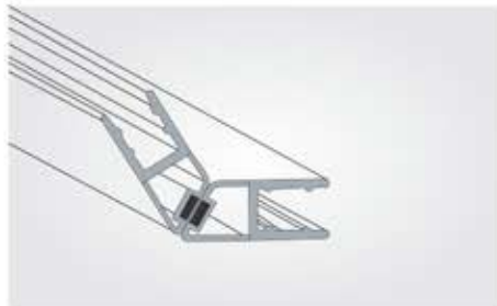
ZPS-M2 135° (Magnetic Seal for 135° Connection) 8mm (2.2mtr.) M.R.P ₹-1050.00 10mm (2.2mtr.) M.R.P ₹-1050.00 12mm (2.2mtr.) M.R.P ₹-1050.00
